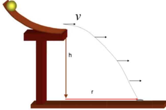
Figure 3: Trajectory of the metal ball.
