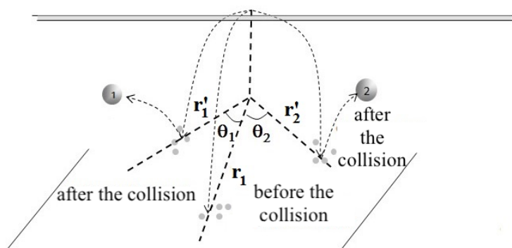
Figure 5: Elastic collision of the balls.
